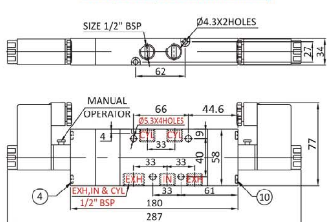
Size : 1/2" BSP (Dimensions are in mm)
