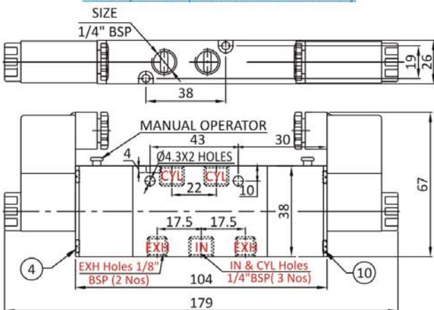
Size : 1/4" BSP (Dimensions are in mm)
