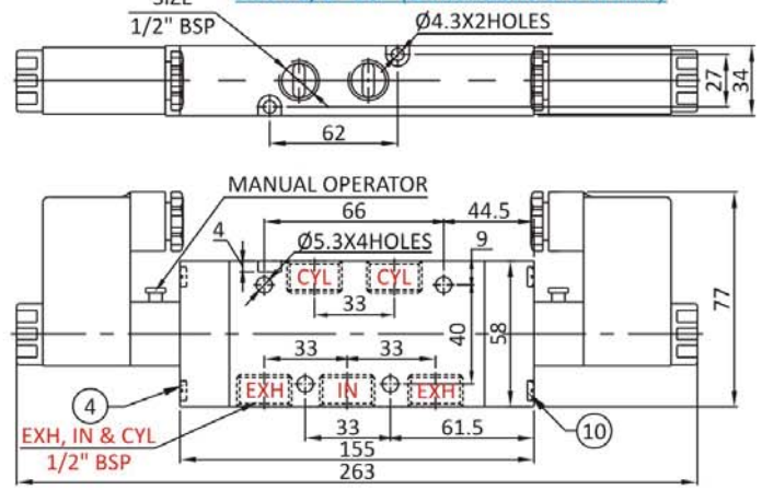
Size : 1/2" BSP (Dimensions are in mm)
