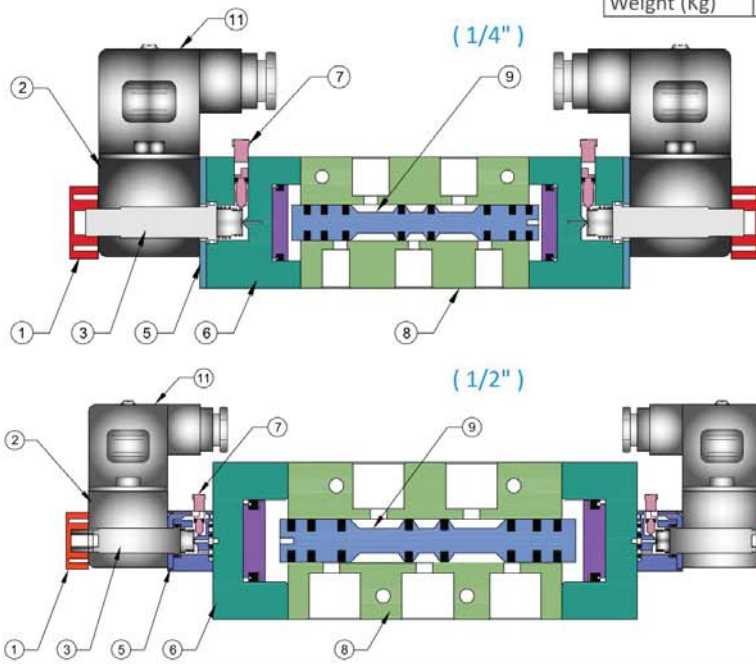
Size : 1/4" BSP (Dimensions are in mm)
