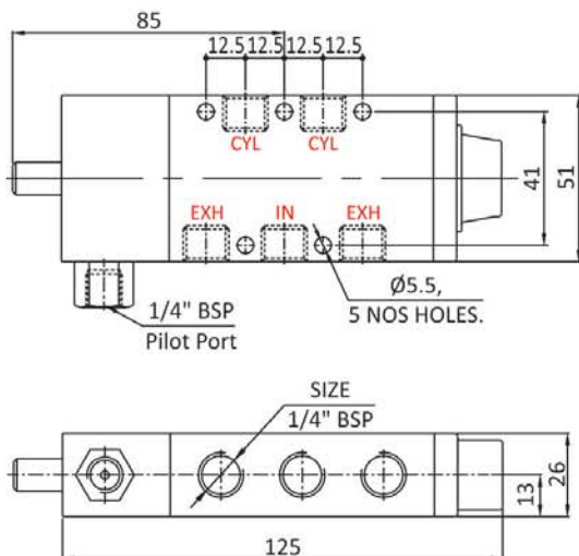
Size : 1/4" BSP (Dimensions are in mm)
