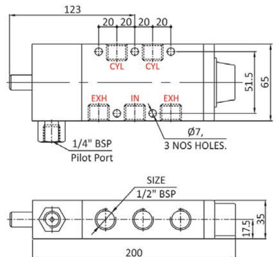
Size : 1/2" BSP (Dimensions are in mm)
